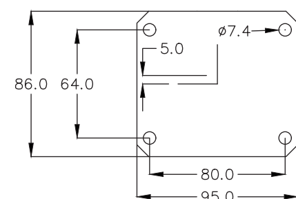
103偏心平板尺寸 103 Series Eccentric Plate
