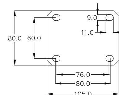
103平板尺寸 103 Series Top Plate
